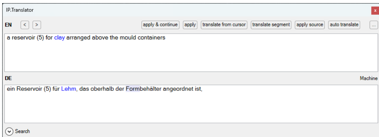
Fig. 14: The translation pop-up window
