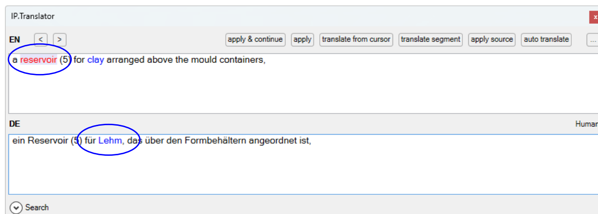
Fig. 24: Examples of glossary entry matching (blue: matching translation, red: no match)
