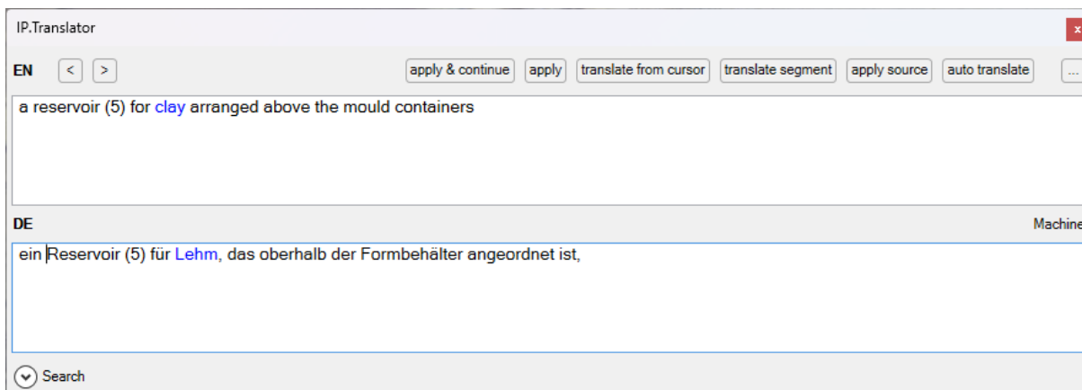
Fig. 17: Translation pop-up window before manual adaptation of DE text; blue text marks matched glossary entry
