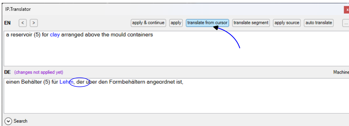
Fig. 18: Translation pop-up window after change in DE text and translation from cursor, blue ellipsis marks syntactical adaptation
