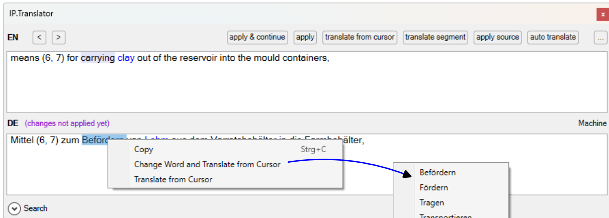
Fig. 19: Translation pop-up window with translation suggestion after right click on selected term
